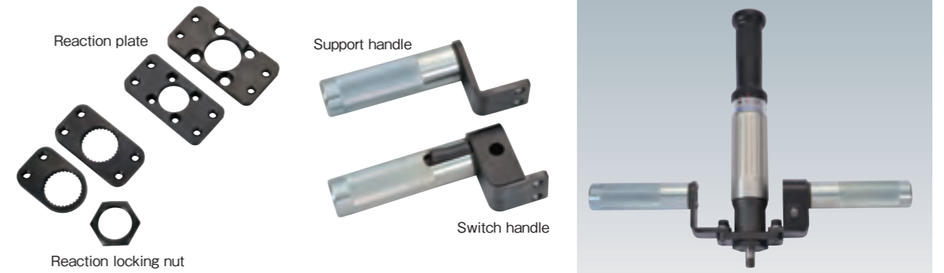
An example of the handle installation
